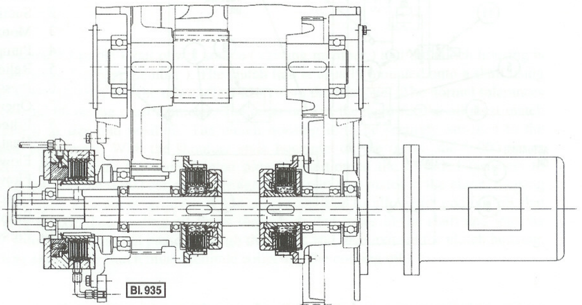
Drive system for a 100 Hp mooring winch, fitted with two hydraulically actuated Ortlinghaus Sinus® multi-plate clutches and a hydraulically released spring-applied brake series 0-022.
