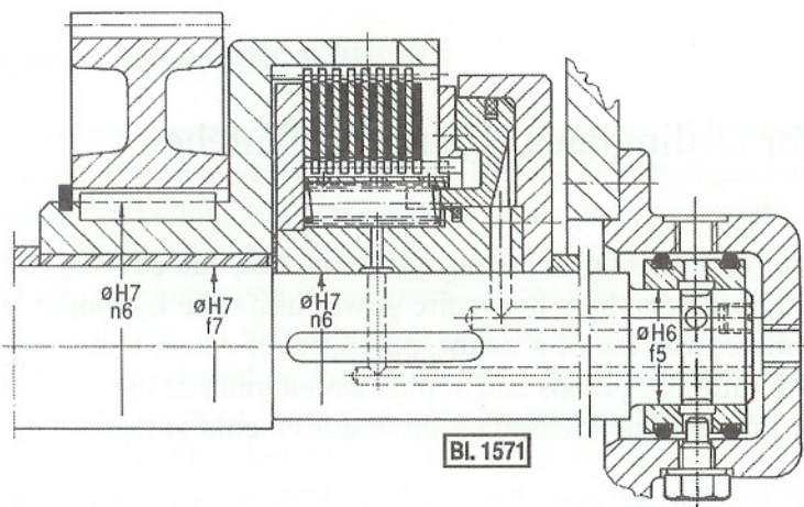
Hydraulically actuated Ortlinghaus Sinus® multi-plate clutch hub housing with plain bearing.
