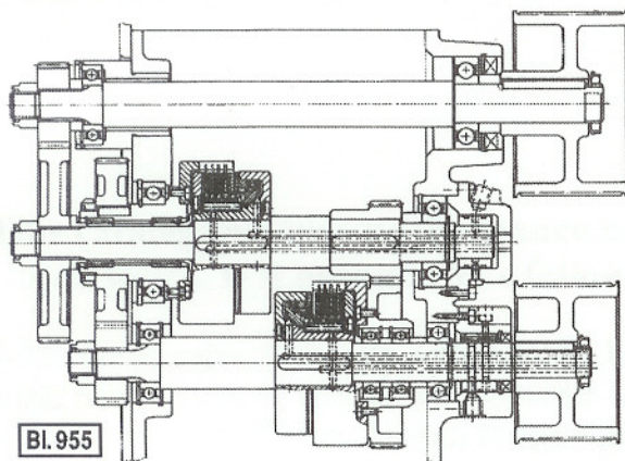
Hydraulically actuated Ortlinghaus Sinus® multi-plate clutches in a gearbox.
